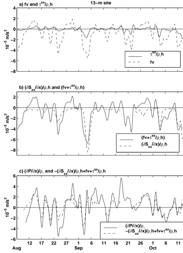
Figure 10. Time series of largest terms in the cross-shelf momentum balance at the 13-m site, (a) Coriolis force f\tilde{v} and wind stress \tau^{sx}/\rho_o h , (b) radiation stress gradient (\rho_o h)^{-1}\partial S_{xx}/\partial x and (f\tilde{v} + \tau^{sx}/\rho_o h) , and (c) pressure gradient \rho_o^{-1}\partial P/\partial x and (f\tilde{v} + \tau^{sx}/\rho_o h - (\rho_o h)^{-1}\partial S_{xx}/\partial x) . Correlations and regression coefficients are given in Table 5.
