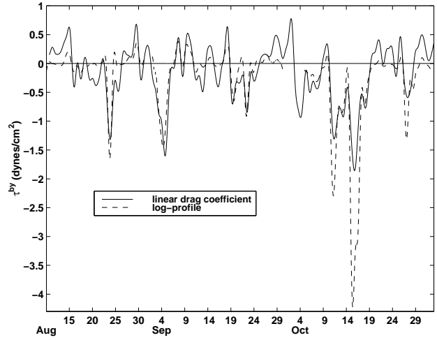
Figure A1. Time series of along-shelf bottom stress at the 21-m site estimated using a linear drag law with r = 5 \times 10^{-4}\text{ m/s} and log-profiles from either a bottom tripod or a bottom tetrapod. Tetrapod-based estimates are shown during August, when a tripod and tetrapod were both deployed.
