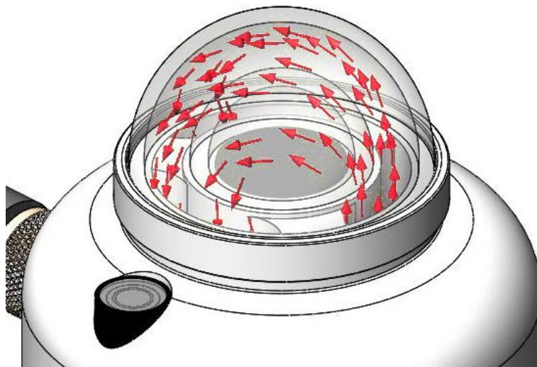
Figure 2.0.4 Recirculating ventilation and heating between the inner- and outer dome is much more power-efficient than traditional ventilation systems.
