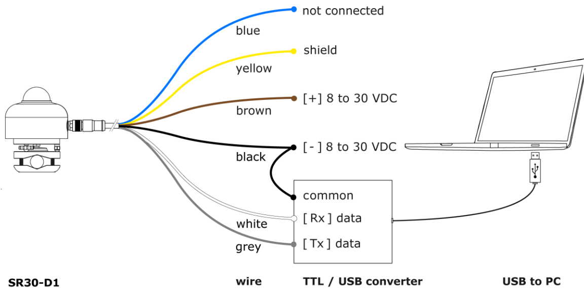
Figure 6.8.1 Connecting SR30-D1 to an RS-485 to USB converter and a PC
