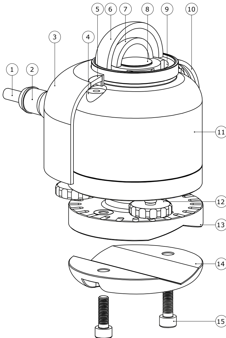
Figure 2.0.1 Overview of SR30-D1:
