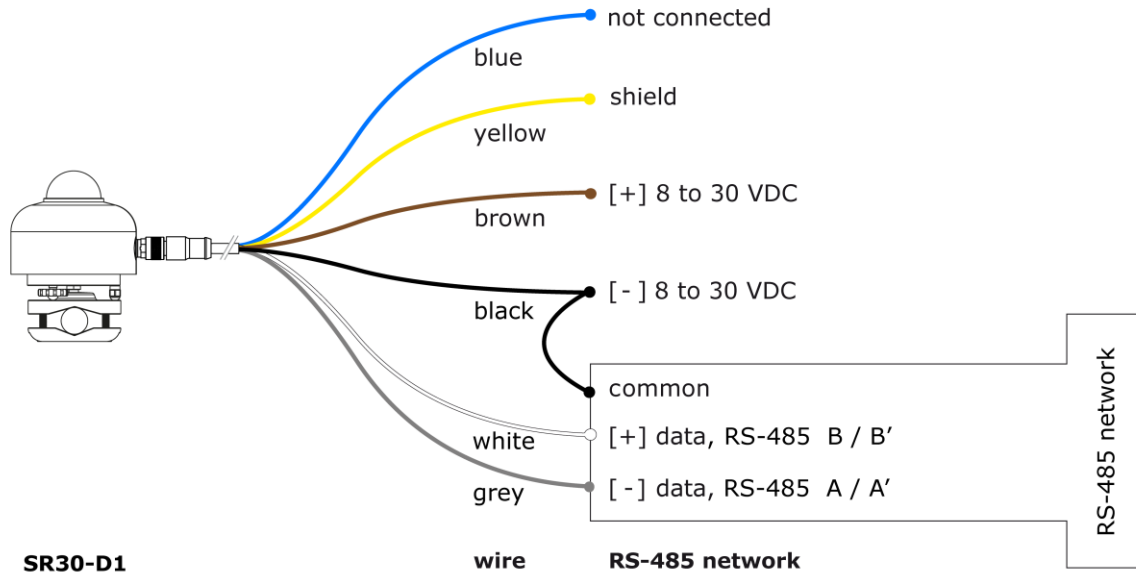
Figure 6.7.2 Connection of SR30-D1 to an RS-485 network. SR30-D1 is powered by an external power supply of 8 to 30 VDC.
