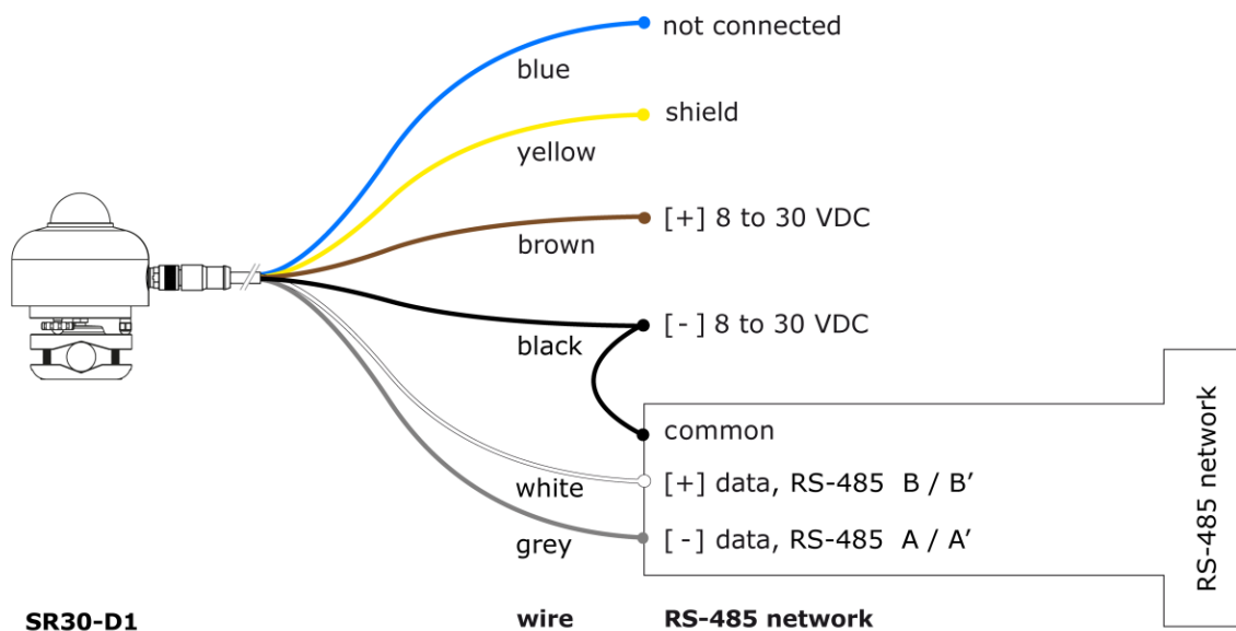
Figure 7.3.1 Connecting SR30-D1 to a typical RS-485 network
