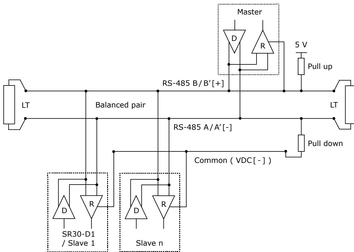
Figure 6.7.1 Typical topology of a two-wire RS-485 network, figure adapted from: Modbus over serial line specification and implementation guide V1.02 (www.modbus.org) . The power supply is not shown in this figure.
