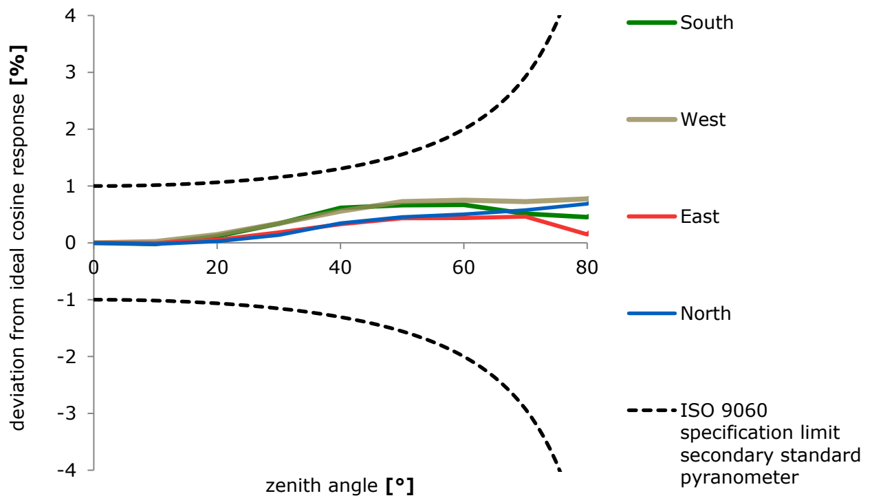
Figure 2.0.3 Directional response of an SR30-D1 pyranometer of 4 azimuth angles, compared to secondary standard limits.
