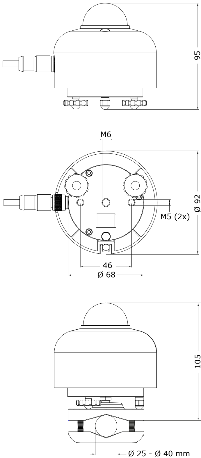
Figure 3.2.1 Dimensions of SR30-D1 in \times 10^{-3} m. Mounts are optional
