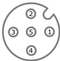
Figure 6.5.1: Connector layout of SR30-D1 indicating PIN numbers (viewed from cable side)
