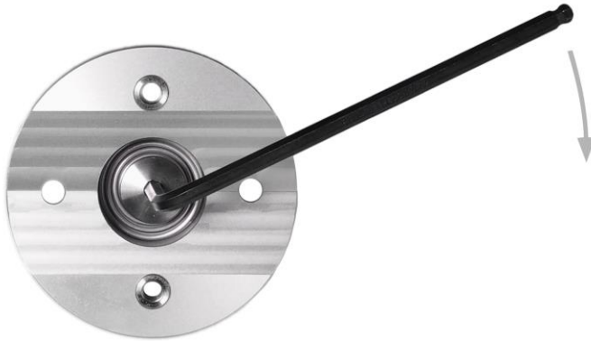
Figure 6.3.1.2 bottom of SR30-D1 levelling mount. Preferred (un)locking with 4 mm hex key
