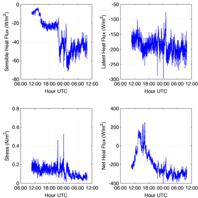
Figure 3.2: Air-Sea fluxes on November 18-19 2006 near Climode 1 buoy.
