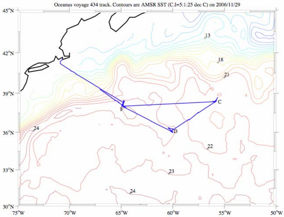
Figure 1.1: Ship's track for Oceanus voyage 434, November 2006. F is surface mooring, C and D are subsurface moorings.
