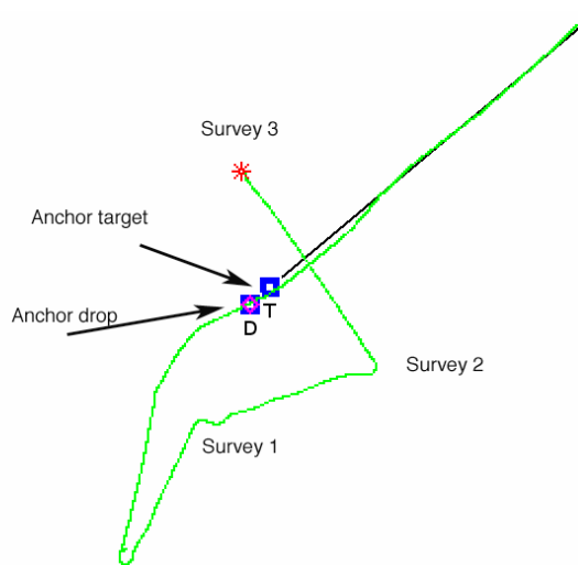
Figure 4.4: Track for anchor survey of Climode 2 mooring D.
