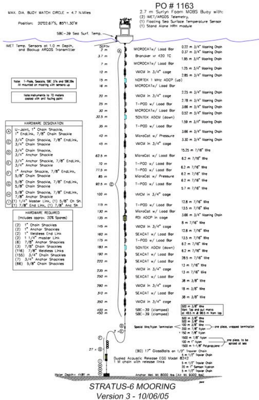
Figure III E.1. Stratus 6 mooring design.
