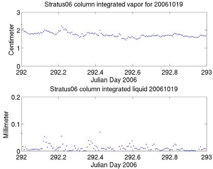
Figure IV.B.11. Time series of data from the Radiometrics microwave radiometer: column water vapor (upper panel), column water liquid (lower panel) for day 292 (October 19, 2006).
