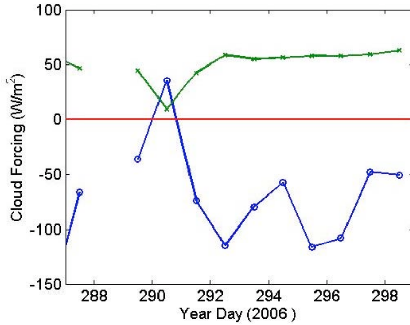
Figure IV.C.6. Time series of daily averaged radiative cloud forcing: IR CF ( \text{W}/\text{m}^2 ) – green, Solar CF ( \text{W}/\text{m}^2 ) – blue. Data for day 288 missing.
