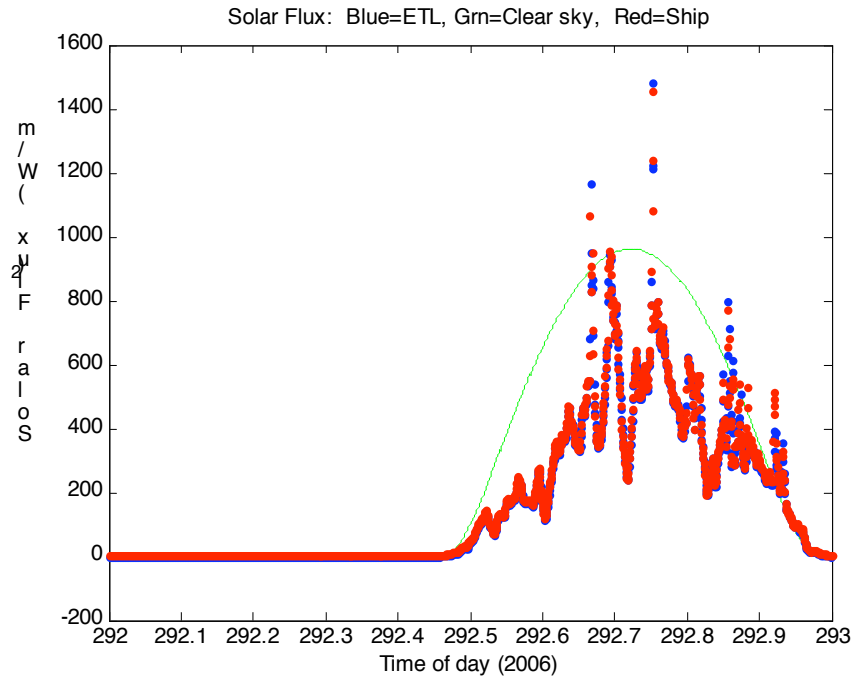
Figure IV.B.5. Time series of downward solar flux from PSD and ship Eppley sensors. The green line is a model of the expected clear sky value.
