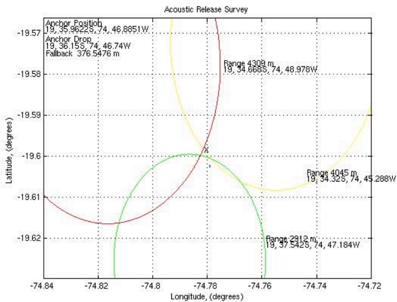
Figure VI.C.8. DART II anchor triangulation using ECours.
