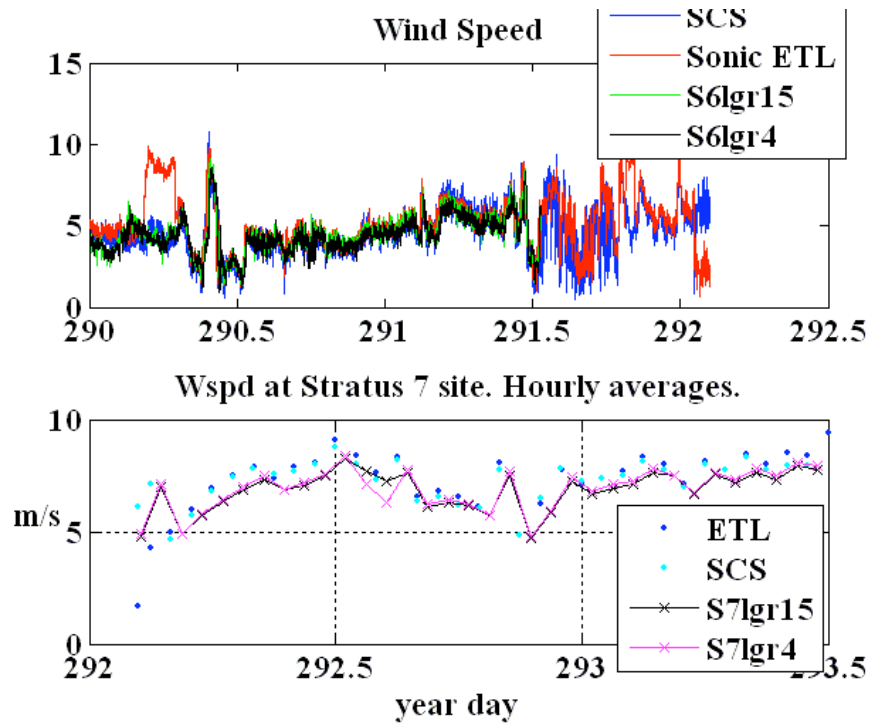
FigureV.B.13. Wind speed data comparison.
