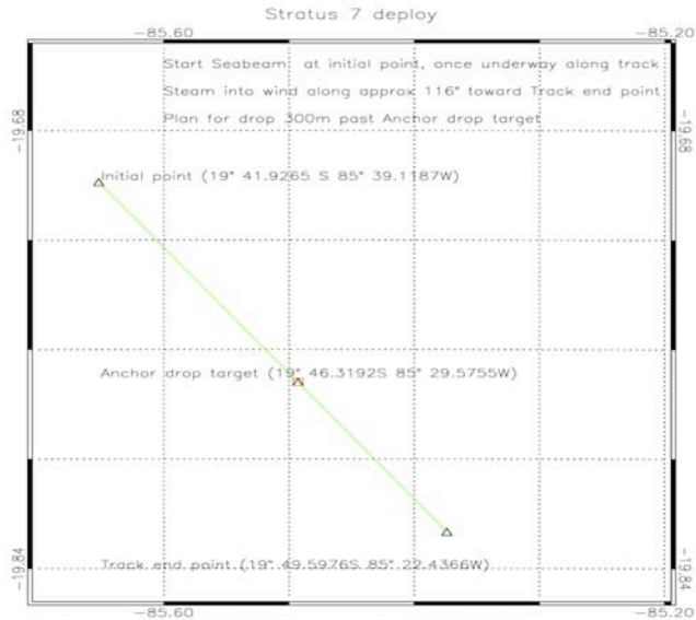
Figure III.D.4. Track used for the deployment of Stratus 7.
