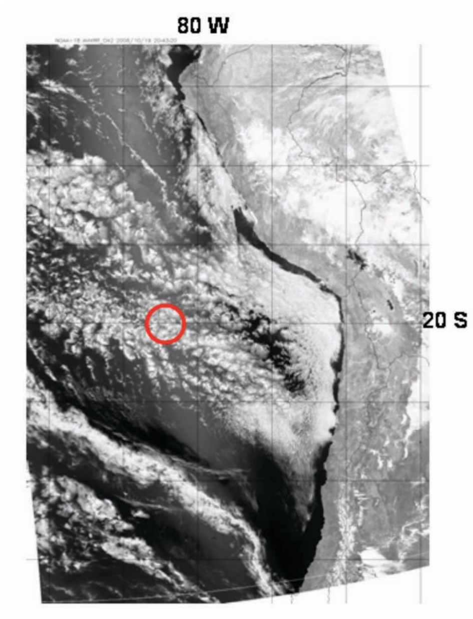
Figure IV.C.18. Terascan satellite visible image NOAA-18 2043 UTC October 19, 2006. Red circle is the location of the STRATUS buoy (20 S, 85W)
