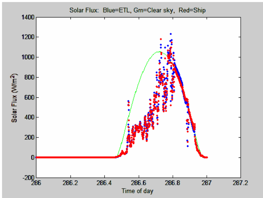
Figure 14. Time series of downward solar flux from ETL and ship Eppey sensors. The green line is a model of the expected clear sky value.
