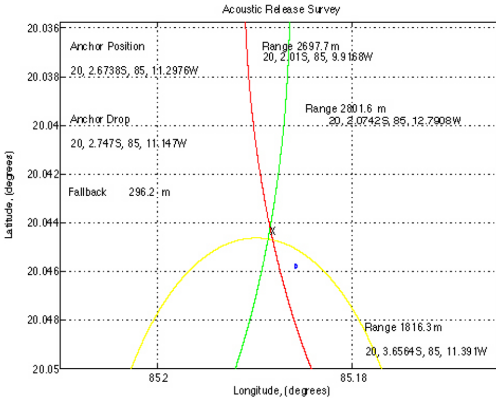
Figure 9. The horizontal range arcs and anchor position (20° 2.6738'S, 85° 11.2975'W) determined using Ccours.
