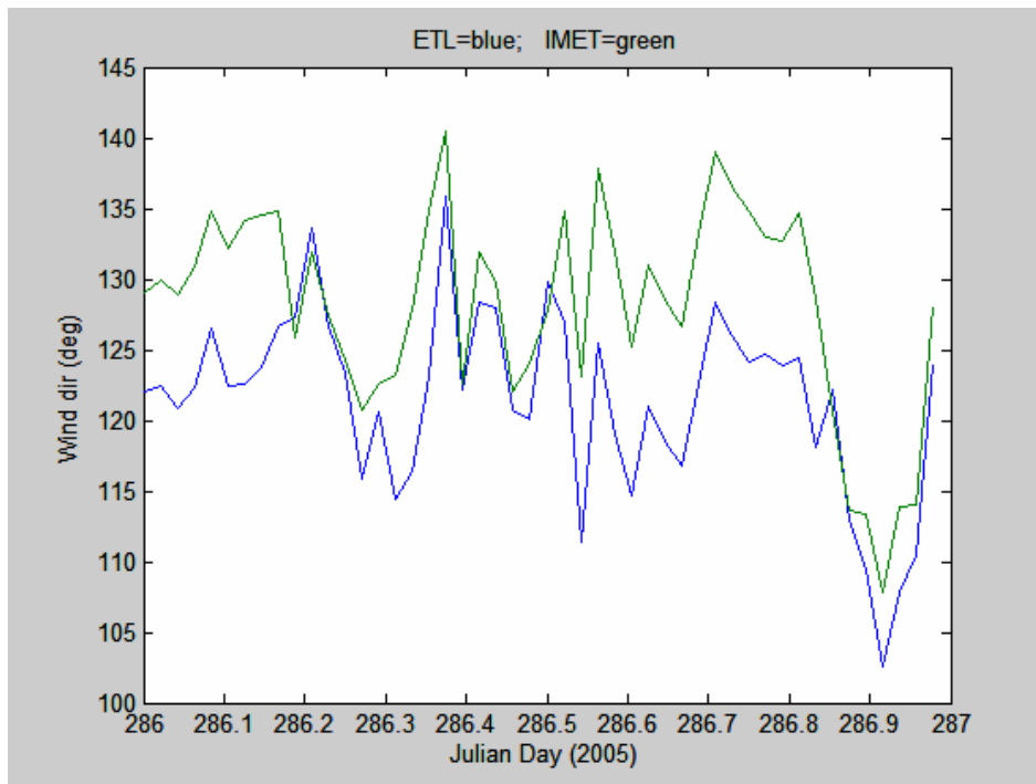
Figure 12. True wind direction from the ETL sonic anemometer (18 m) and the IMET propvane (15 m).
