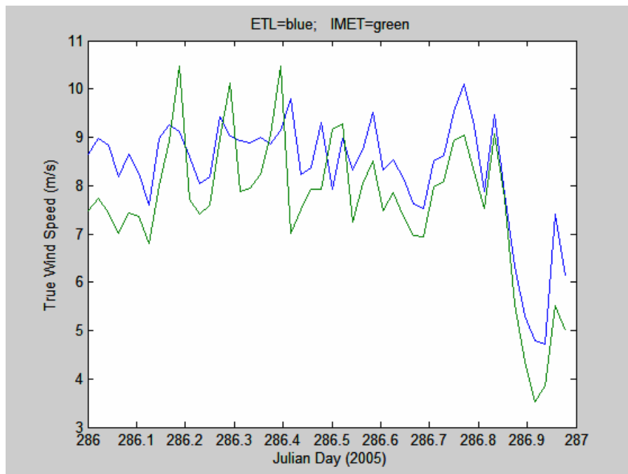
Figure 13. True wind speed from the ETL sonic anemometer (18 m) and the ship's propvane (15 m).
