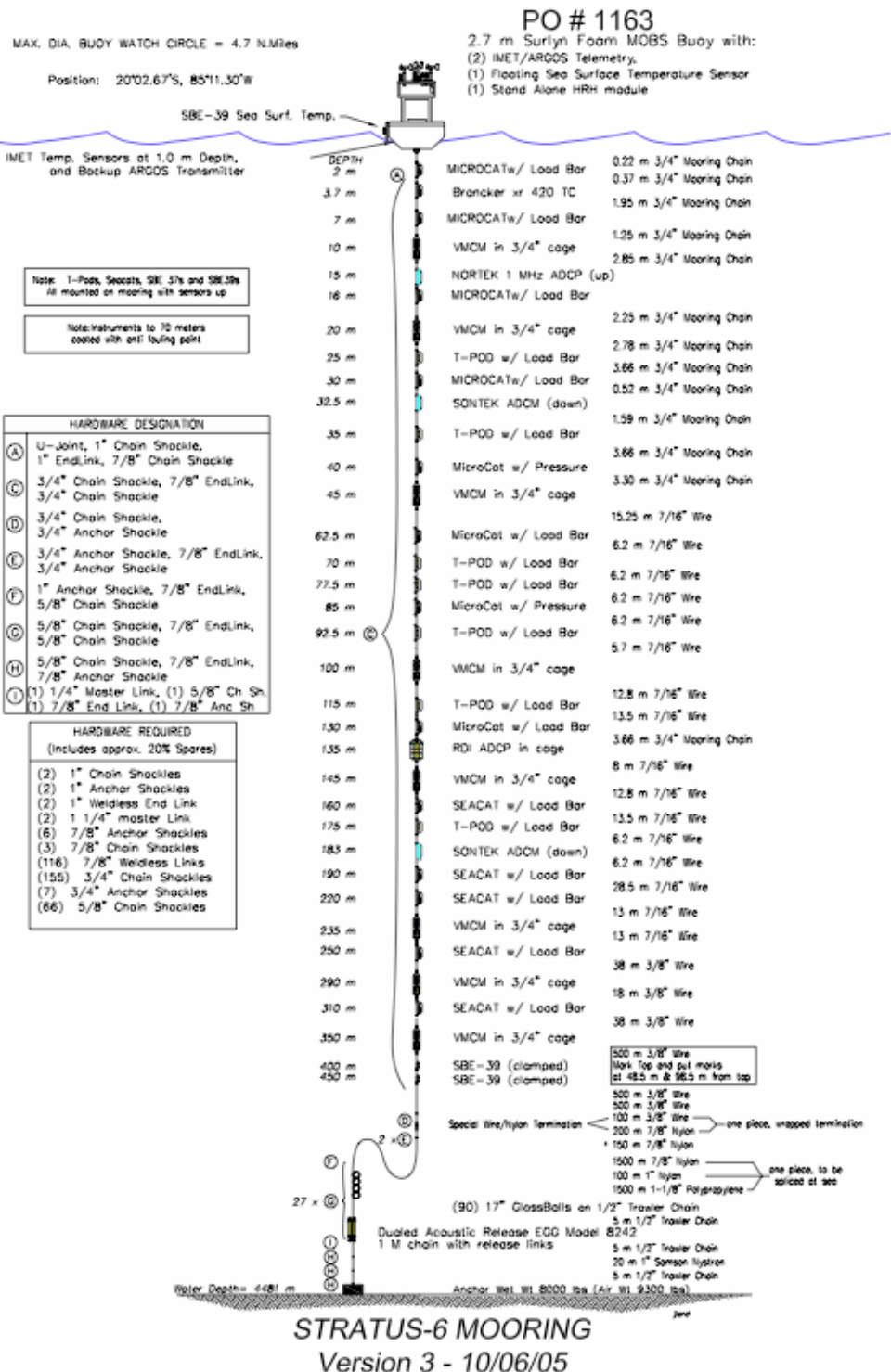
Figure 3: The Stratus 6 mooring diagram
