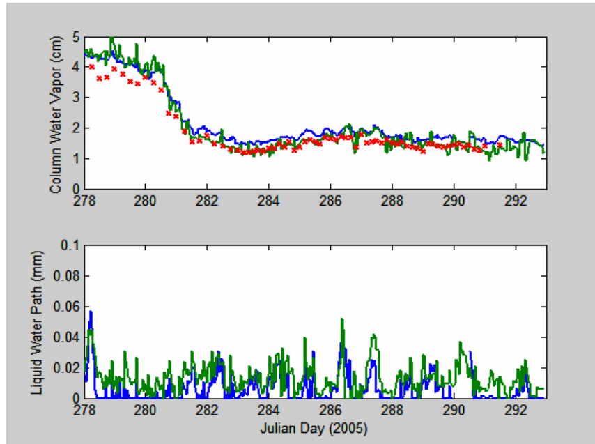
Figure 36. Time series of microwave radiometer-derived values for column integrated water vapor (upper panel) and column integrated liquid water (lower panel). Old mailbox=green, new mailbox=blue, and integrals from rawinsonde profiles=red x's (upper panel only).
