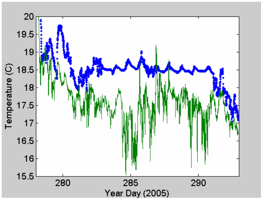
Figure 24. Time series of near-surface ocean temperature (blue) and 15-m air temperature (green) for the 2005 RHB Stratus cruise.
