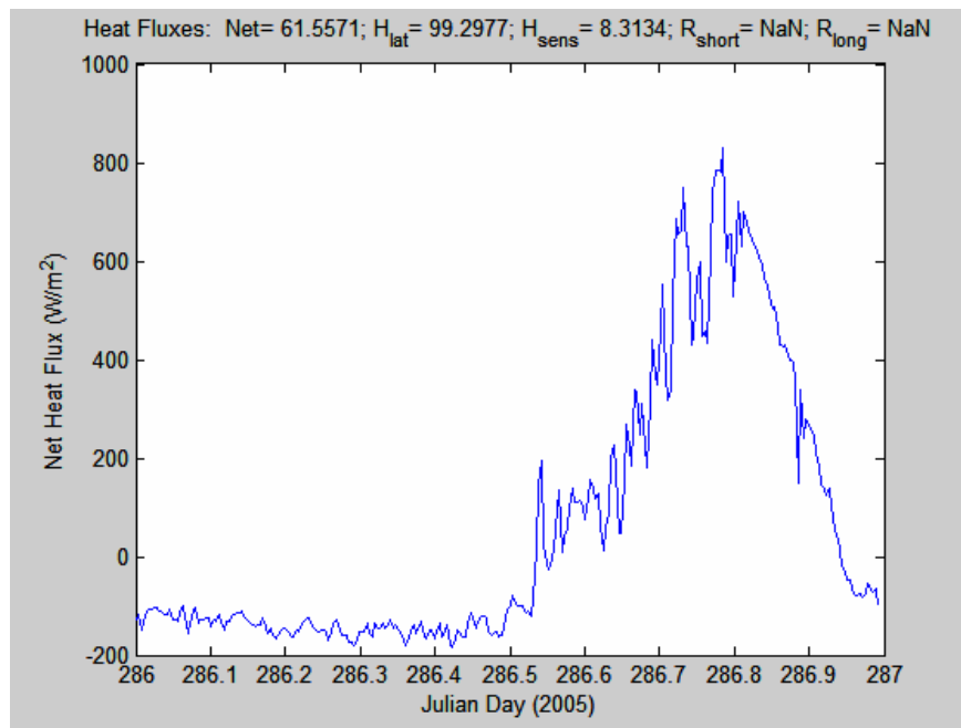
Figure 17. Time series of net heat flux to the ocean surface. The values at the top of the graph are the average for the day for each component of the flux.
