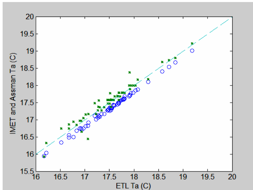
Figure 37. Comparison of simultaneous Assman psychrometer (x's) and ship (circles) readings for air temperature. Psychrometer values corrected to 15 m (ETL and ship instrument height).
