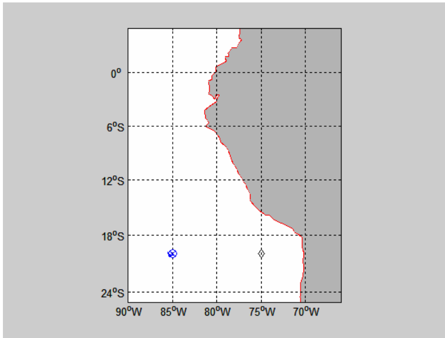
Figure 10. Cruise track for RBH on October 13 (DOY 286). The x marks the WHOI buoy location; the diamond is the DART buoy.
