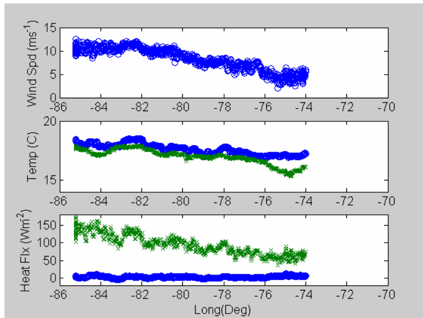
Figure 30. Same as Figure 20, but for the W-E transect along 20° S from 85° W to 70° W.
