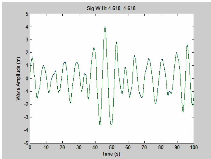
Figure 21. Sample wave time series from 1000 UTC on day 286 (October 13) from the laser rangefinder. The trace shows elevation of the sea surface relative to the bow of the ship. The dominant wave period is about 6 seconds.
