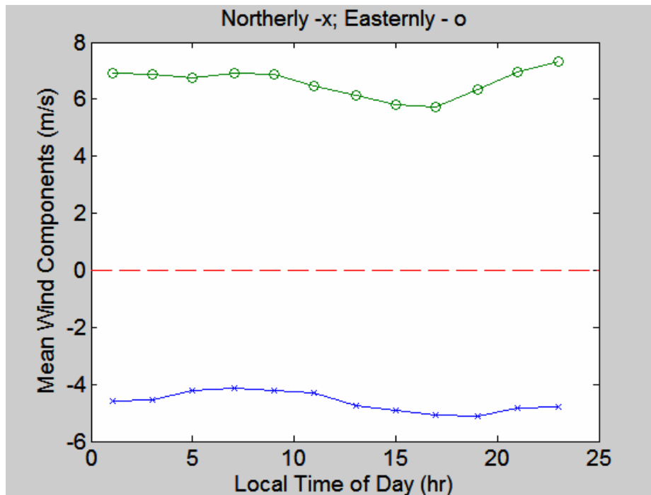
Figure 26. Diurnal average of northerly and easterly wind components for period near 20° S, 85° W.
