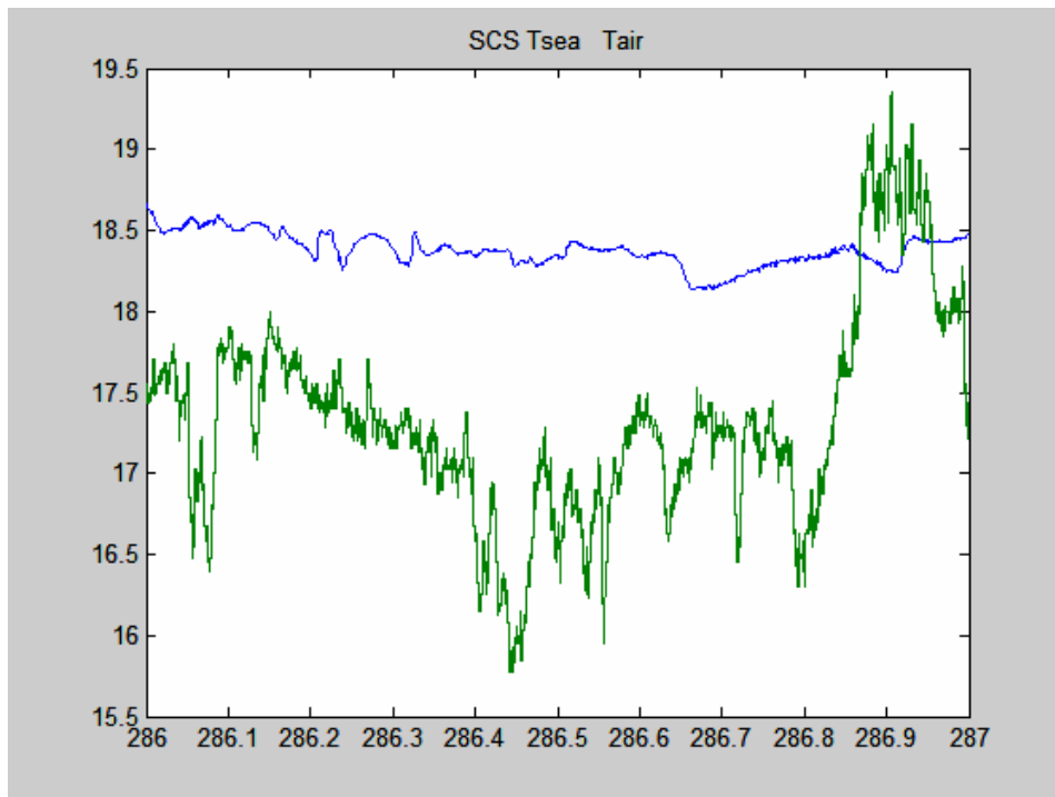
Figure 11. Time series of near-surface ocean temperature (green) and 15-m air temperature (blue).
