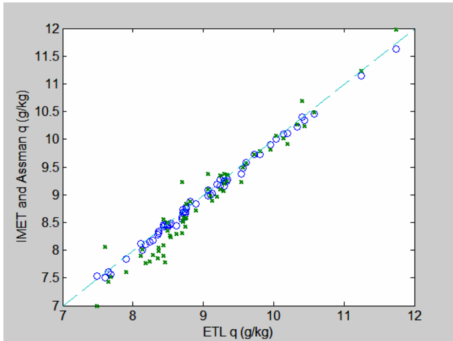
Figure 38. Comparison of simultaneous Assman psychrometer (x's) and ship (circles) readings for specific humidity. Psychrometer values corrected to 15 m (ETL and ship instrument height).
