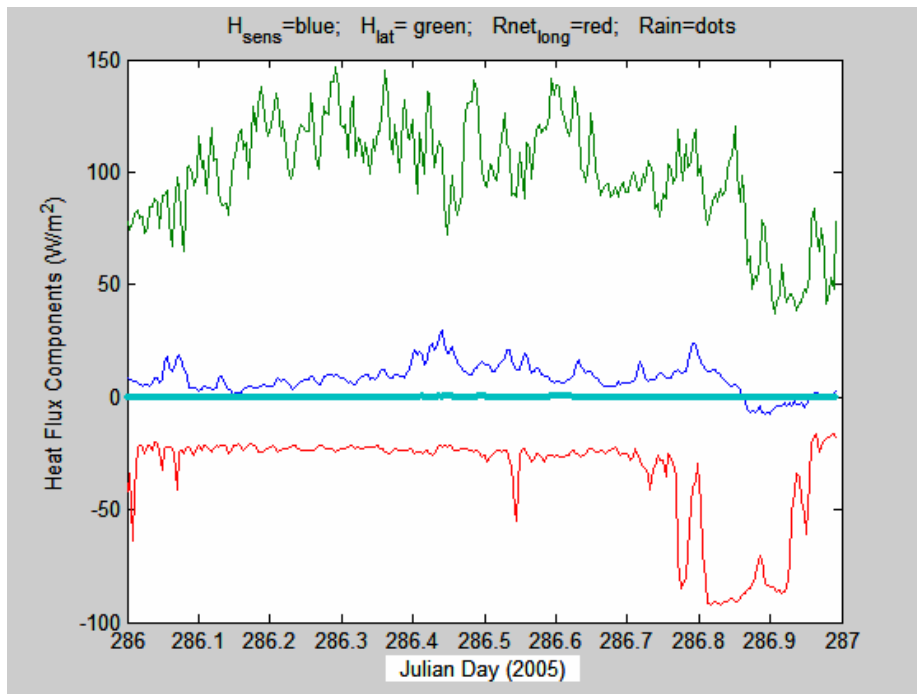
Figure 16. Time series of non-solar surface heat flux components: sensible (blue), latent (green), and net IR (red).
