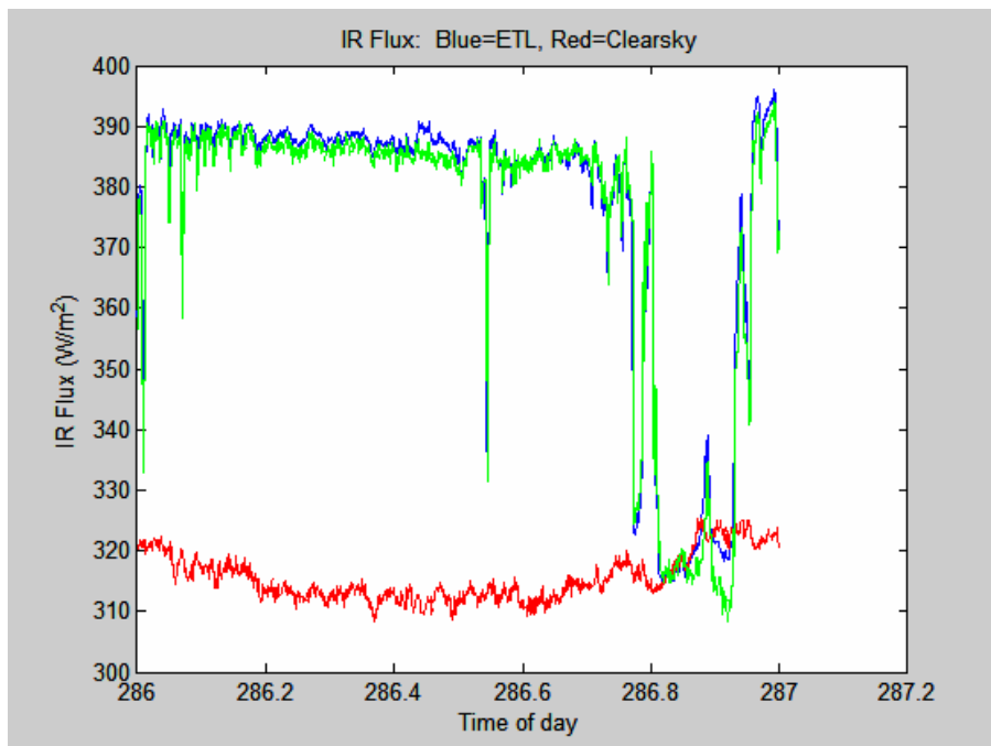
Figure 15. Time series of downward IR flux from ETL and ship Eppey sensors. The red line is a model of the expected clear sky value.
