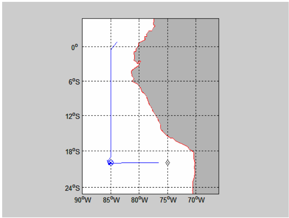
Figure 23. Cruise track for entire Stratus 2005 cruise.
