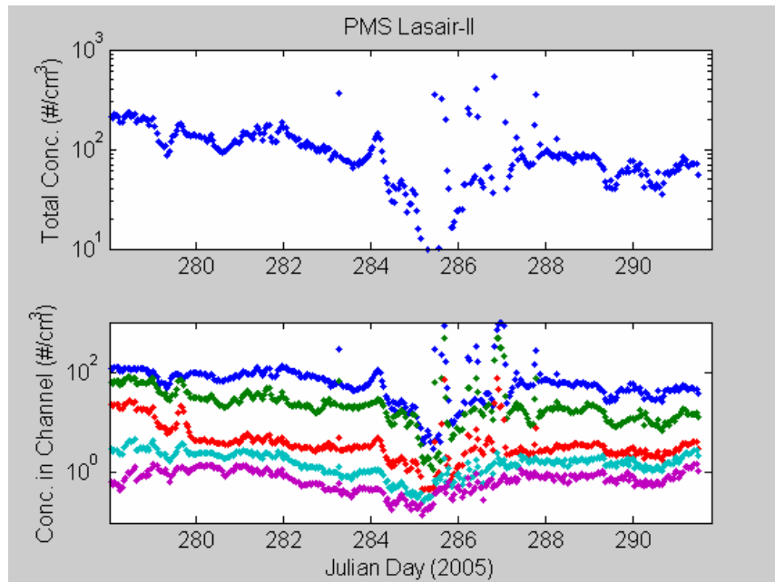
Figure 31. Aerosol concentrations from Lasair-II spectrometer. Upper panel: total number concentration for aerosols larger than 0.1 micron diameter. Lower panel: aerosol concentrations for 0.1-0.2 (blue), 0.2-0.3 (green), 0.3-0.5 (red), 0.5-1.0 (cyan), and 1.0-5.0 (magenta). Spikes are caused by the ship's exhaust.
