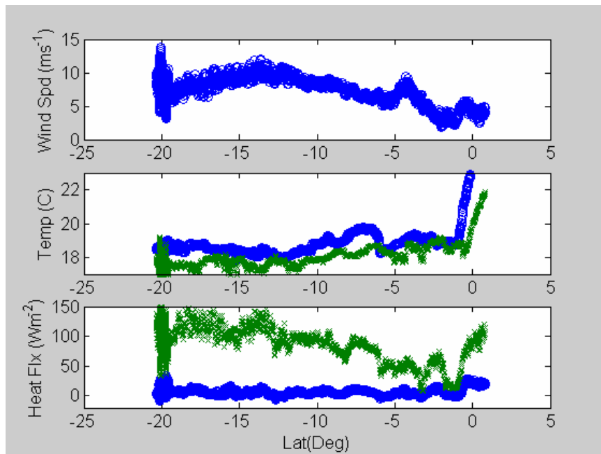
Figure 29. Selected variables from the N-S transect along 85^\circ W. Upper panel is wind speed; the middle panel is sea surface temperature (blue) and air temperature (green); the lower panel shows sensible (blue) and latent (green) heat fluxes.
