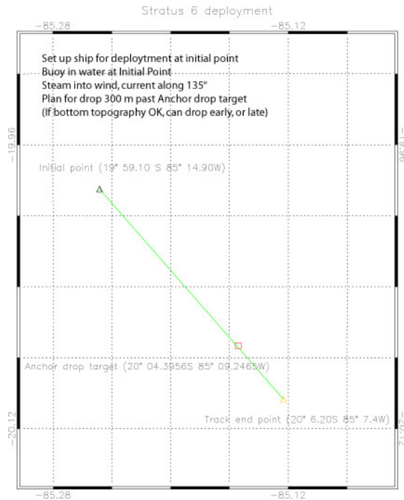
Figure 4. Map showing track plan for Stratus 6 deployment
