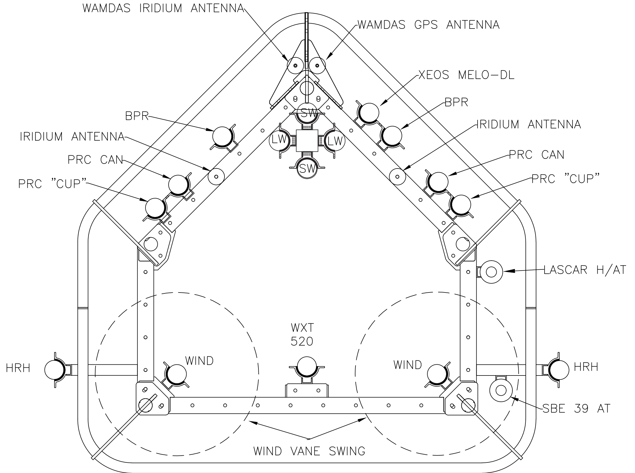
NTAS 12 TOWER TOP As Deployed JL
